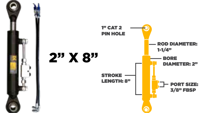
22 - 30" CATEGORY 2 HYDRAULIC TOP LINK KIT 46.230.008
