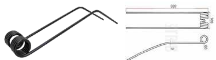
DA ROS GR TINE DA ROS, MODELS GR300/330/380/410 OEM 6900220 45.000.220
