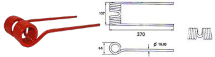
CLAAS LINER N/S RAKE TINE CLAAS 9557100 45.000.710
